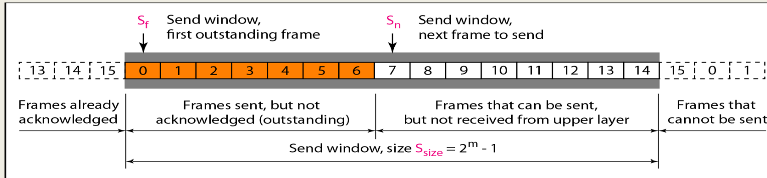
a. Send window before sliding
