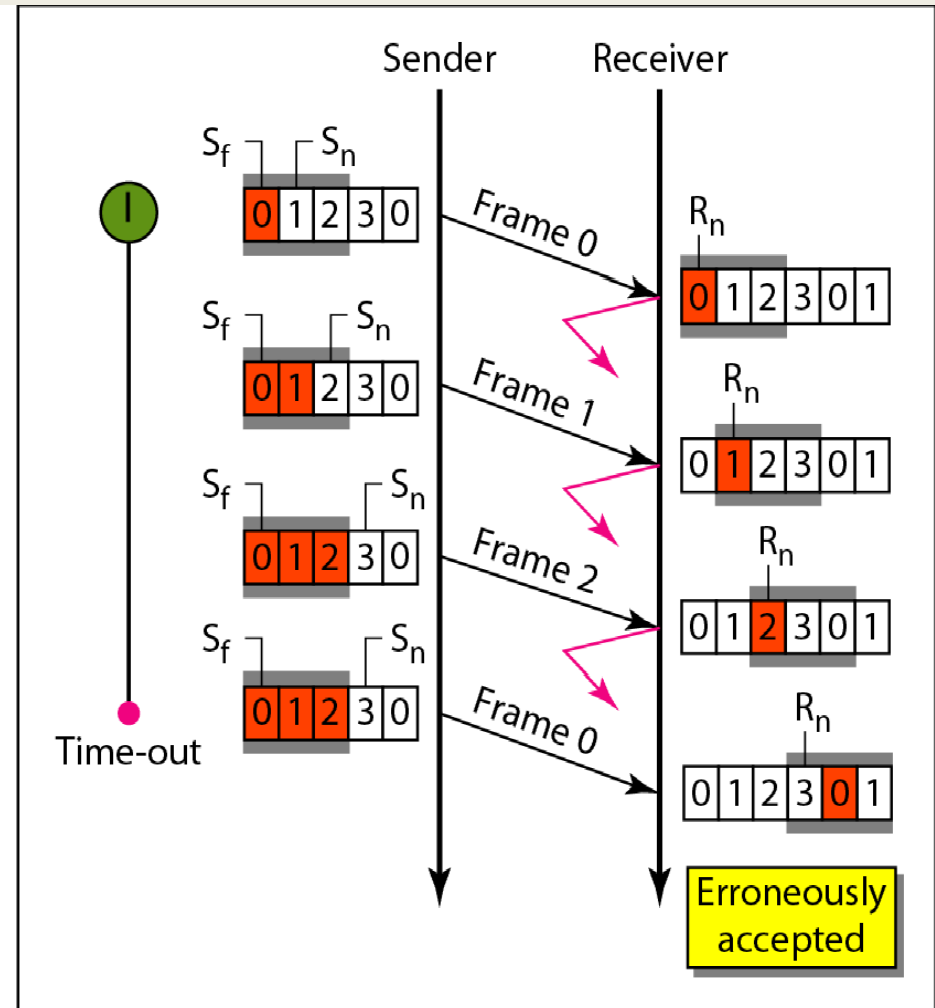
b. Window size > 2^m - 1
